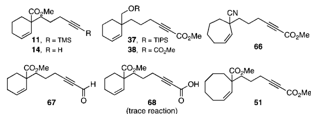
Figure 1. Substrates unreactive to ruthenium catalysis.
