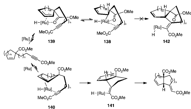
Scheme 12. Alternative Rationale for Cis Diastereoselectivity of 5, n -Systems a
