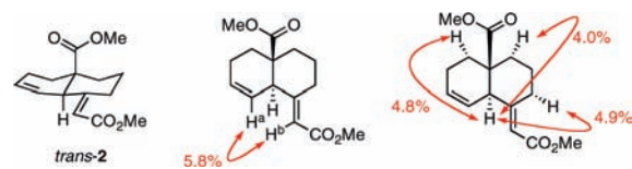
Figure 2. Stereochemical assignment of trans - 2 .
